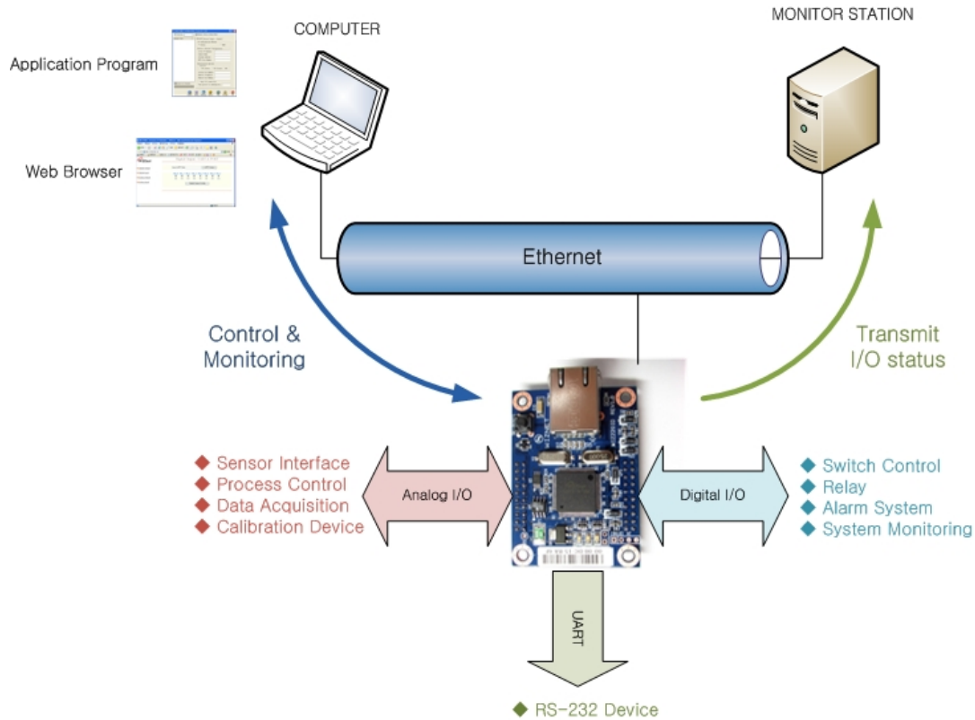
Figure 1. Block Diagram
