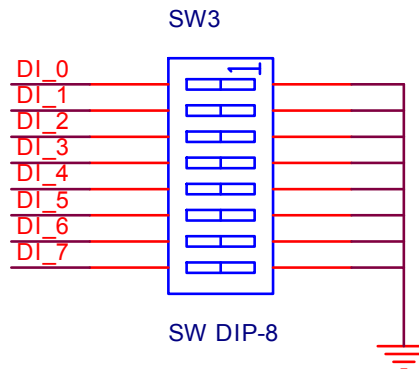
Figure 5. DI Switch of the WIZ220IO Base Board
